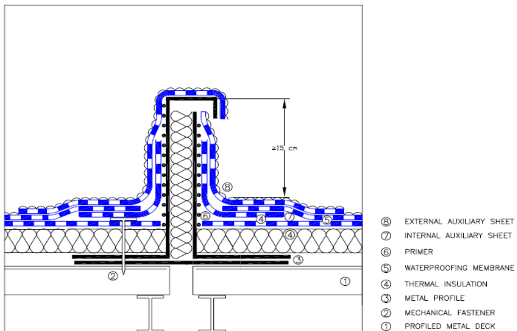
Fig. 2 Detail of a structural joint
