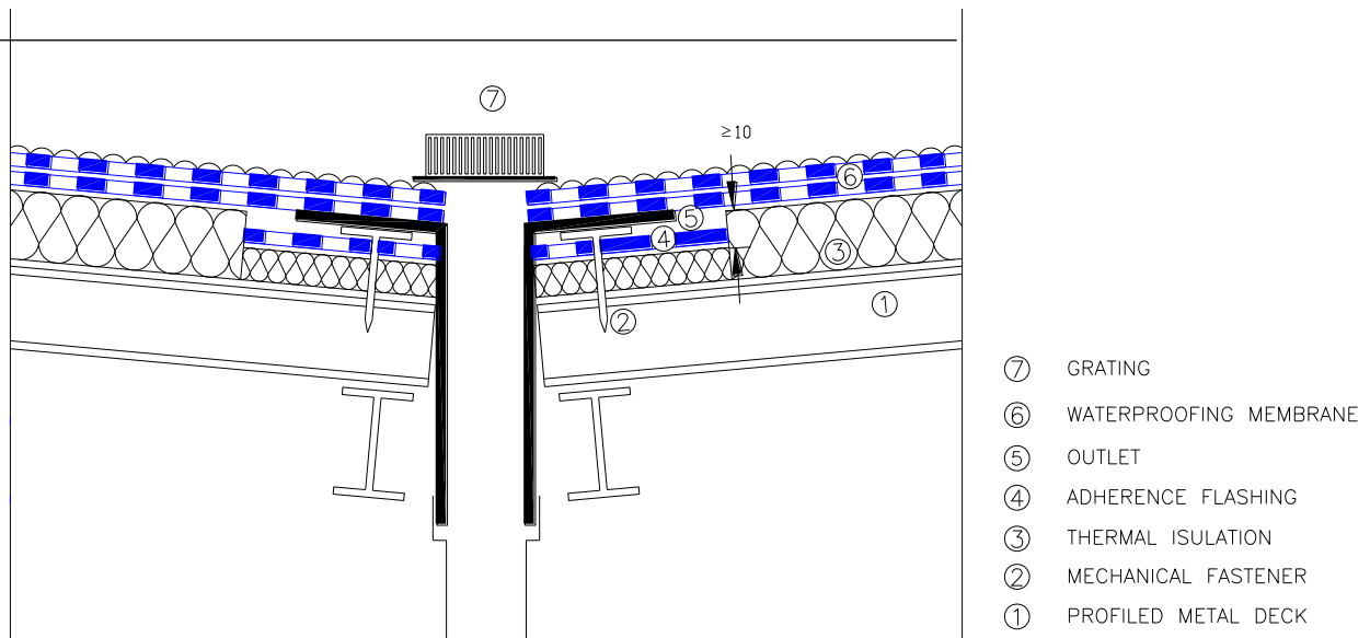
Fig. 4 Drain detail
