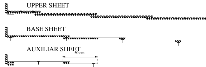
Fig. 6 Reinforcement membrane on valley gutter
