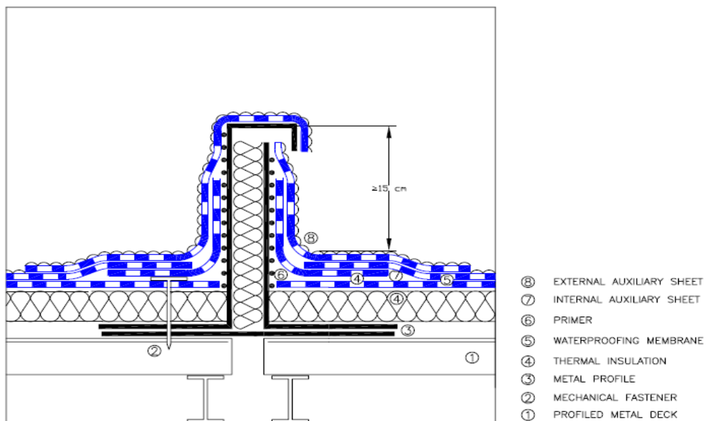
Fig. 2 Detail of a structural joint
